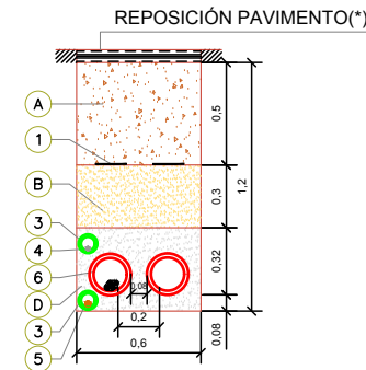
ZANJA TIPO BT (CRUCE) (1 BT)
